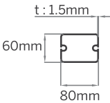
⑤ Puller Profile (Standart)
