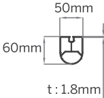
④ Fabric Support (HDD Lux)
